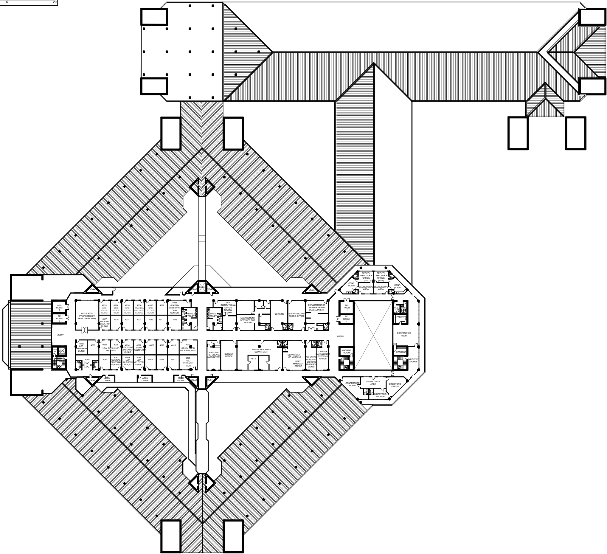
FOURTH FLOOR AS-FOUND PLAN
